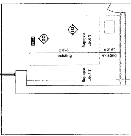
PROPOSED PLAN scale: 1/2" = 1'-0"
