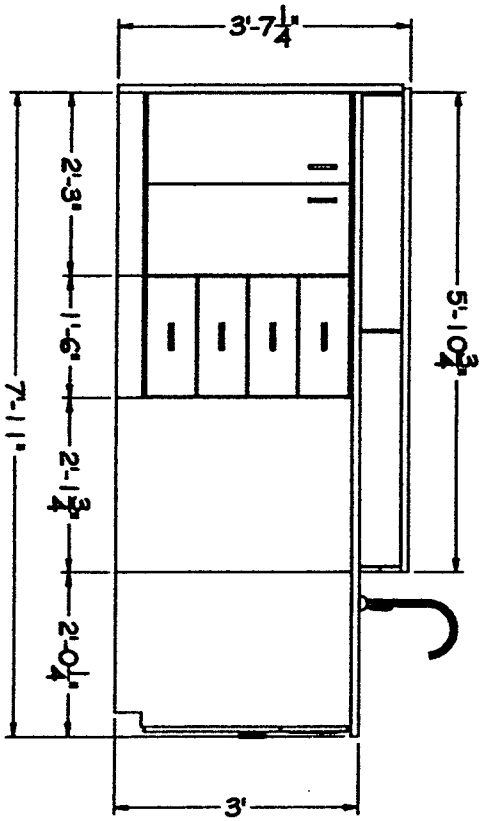
ELEVATION A- TRAINING ROOM TYP. NOT TO SCALE- UTILITY CUTOUTS TO BE MADE ON SITE ALL STORAGE LOCKING
