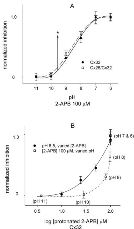
Fig. 2. Inhibition by 2-APB is pH-sensitive. A, inhibition of Cx32 channels (●) and Cx26/Cx32 channels (□) induced by 100 \mu\text{M} 2-APB over a range of pH. The asterisk is the inhibition by 500 \mu\text{M} 2-APB at its pK_a , pH 9.6. B, the protonated form of 2-APB produces the inhibitory effect on Cx32, and protonated connexin modulates the sensitivity. Inhibition is plotted as a function of the concentration of protonated 2-APB using two sets of data: one in which 2-APB was varied at constant pH 6.4 (○, data from Fig. 1A), and one in which the concentration of 2-APB was constant and the pH varied (■, data from Fig. 2A). The difference between the two relations indicate that protonation of connexin enhances the sensitivity of 2-APB. From left to right, the filled squares correspond to 100 \mu\text{M} 2-APB data at pH 11, 10, 9, and 8, with the points at pH 7 and pH 6 superimposed at far right (i.e., for which all 2-APB is protonated). Data points are means \pm S.E. for five protein preparations.
